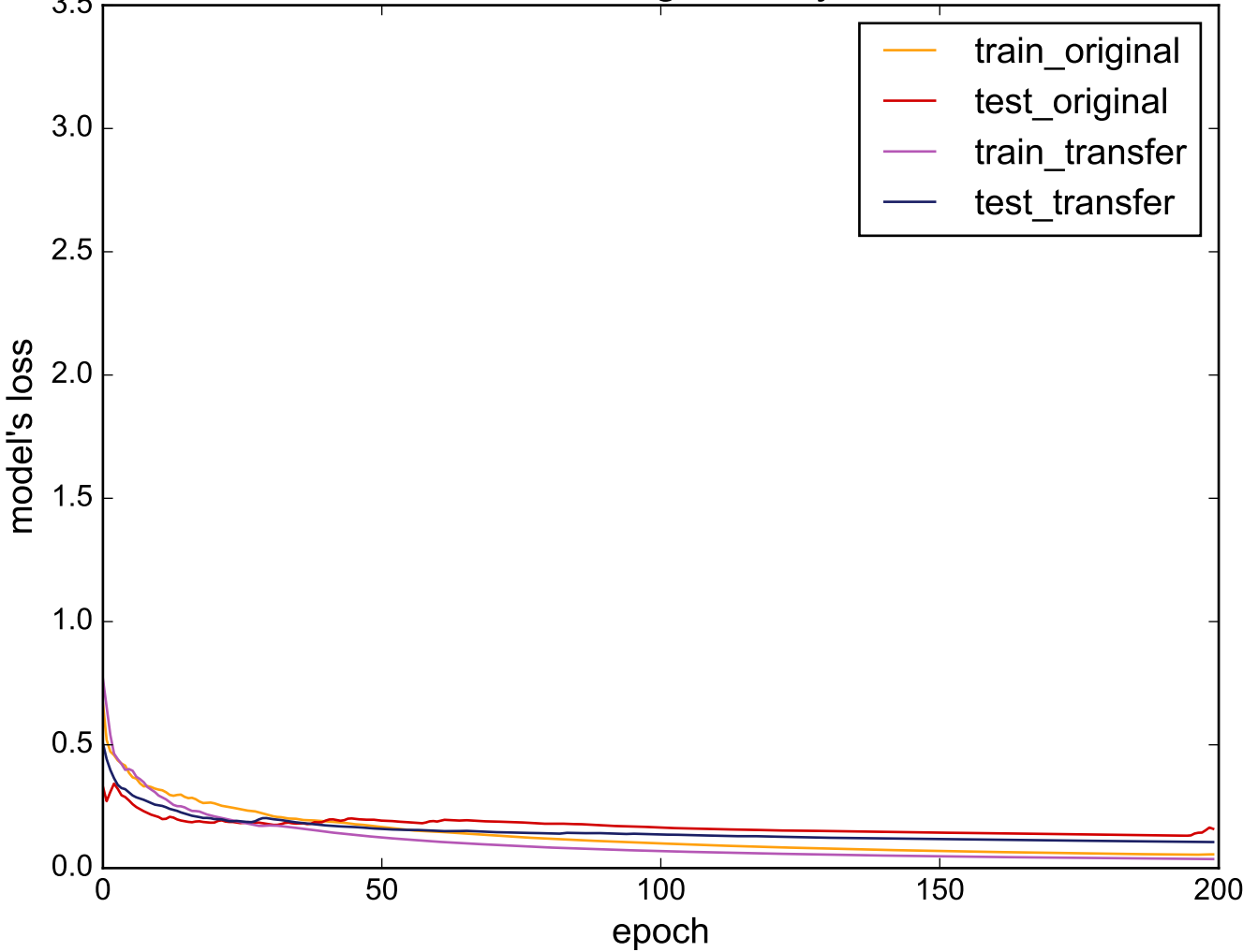
Source: TwoLeadECG - Target: SonyAIBORobotSurface
