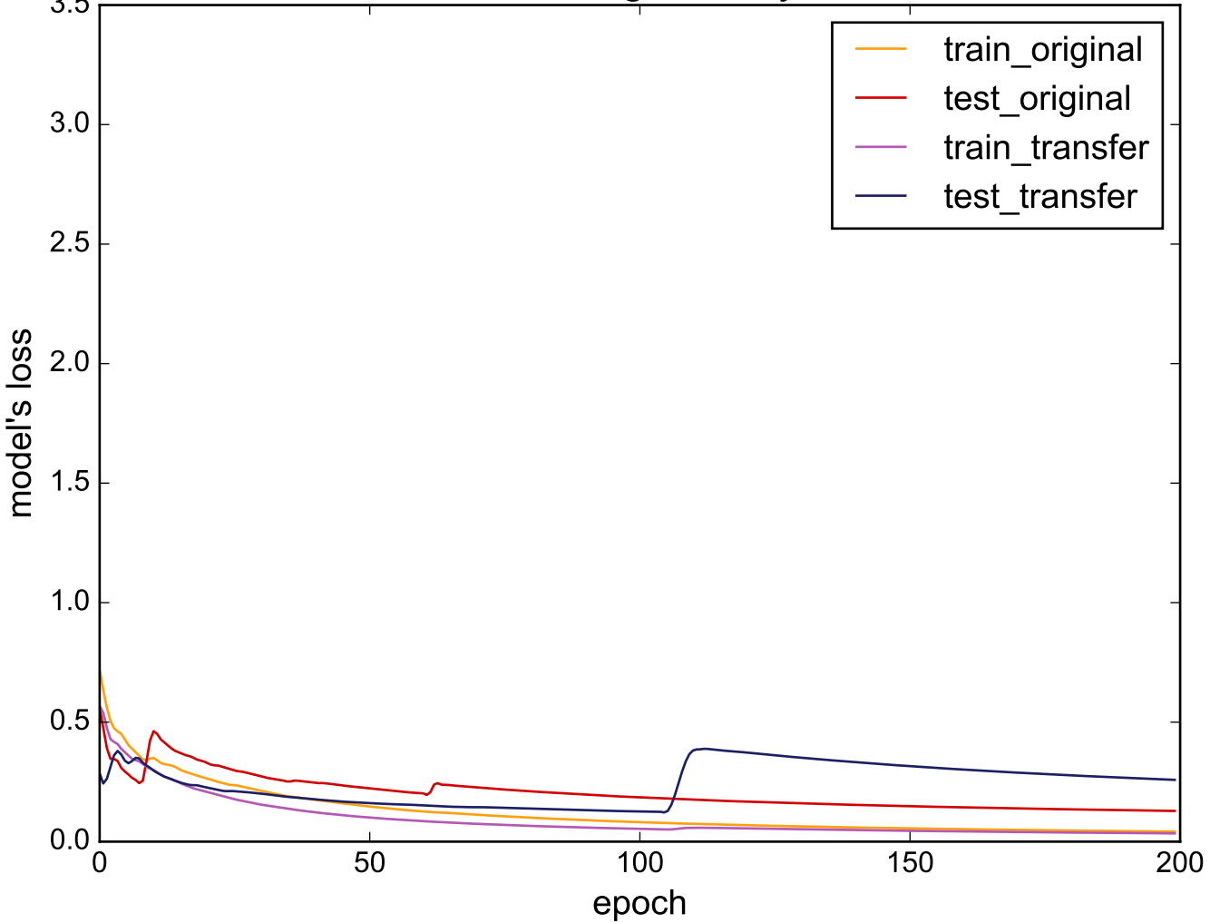
Source: TwoLeadECG - Target: SonyAIBORobotSurfaceII
