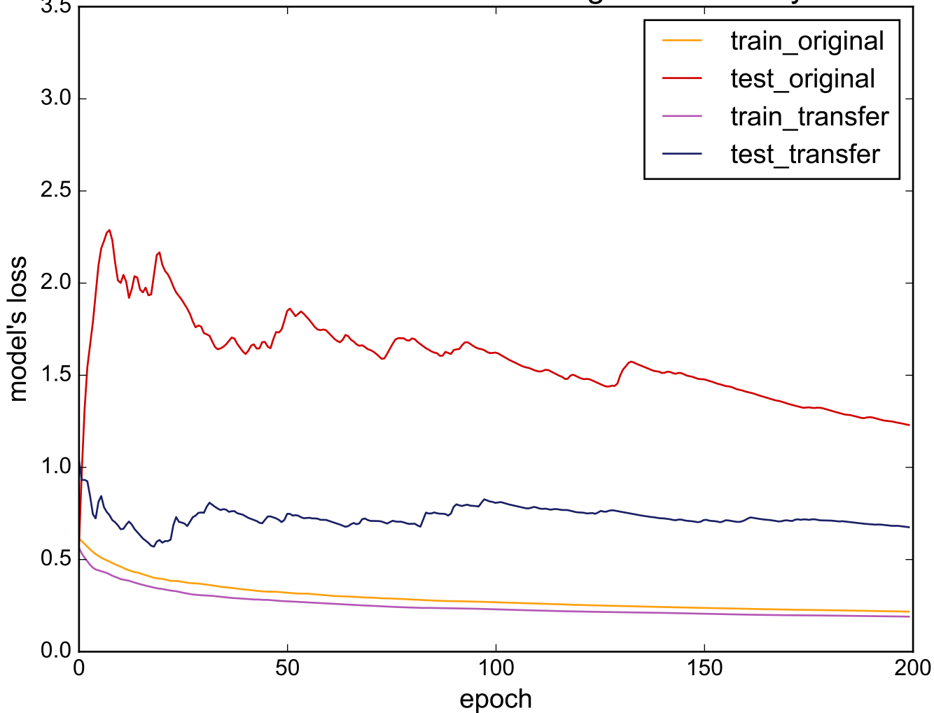
Source: TwoLeadECG - Target: Strawberry
