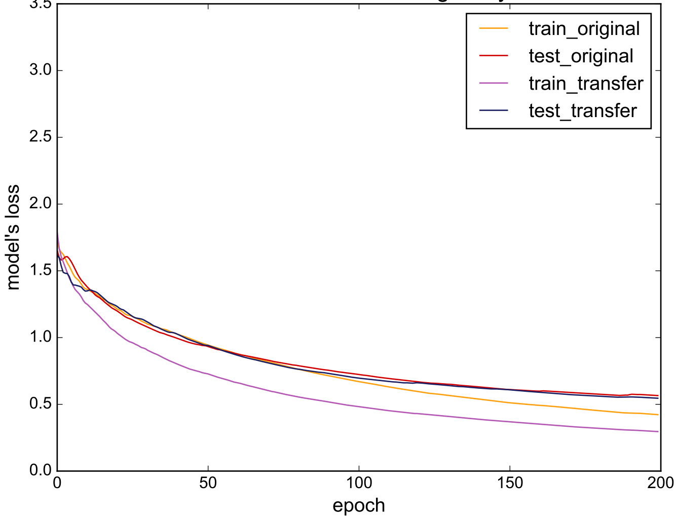
Source: TwoLeadECG - Target: Symbols
