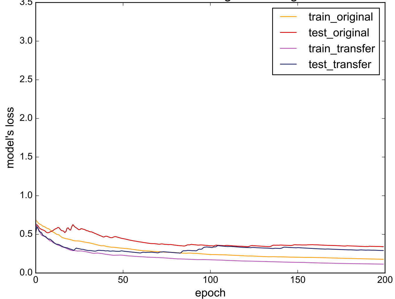
Source: TwoLeadECG - Target: ToeSegmentation1
