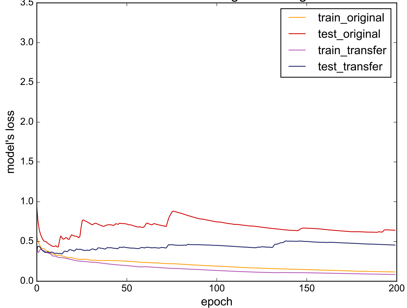
Source: TwoLeadECG - Target: ToeSegmentation2
