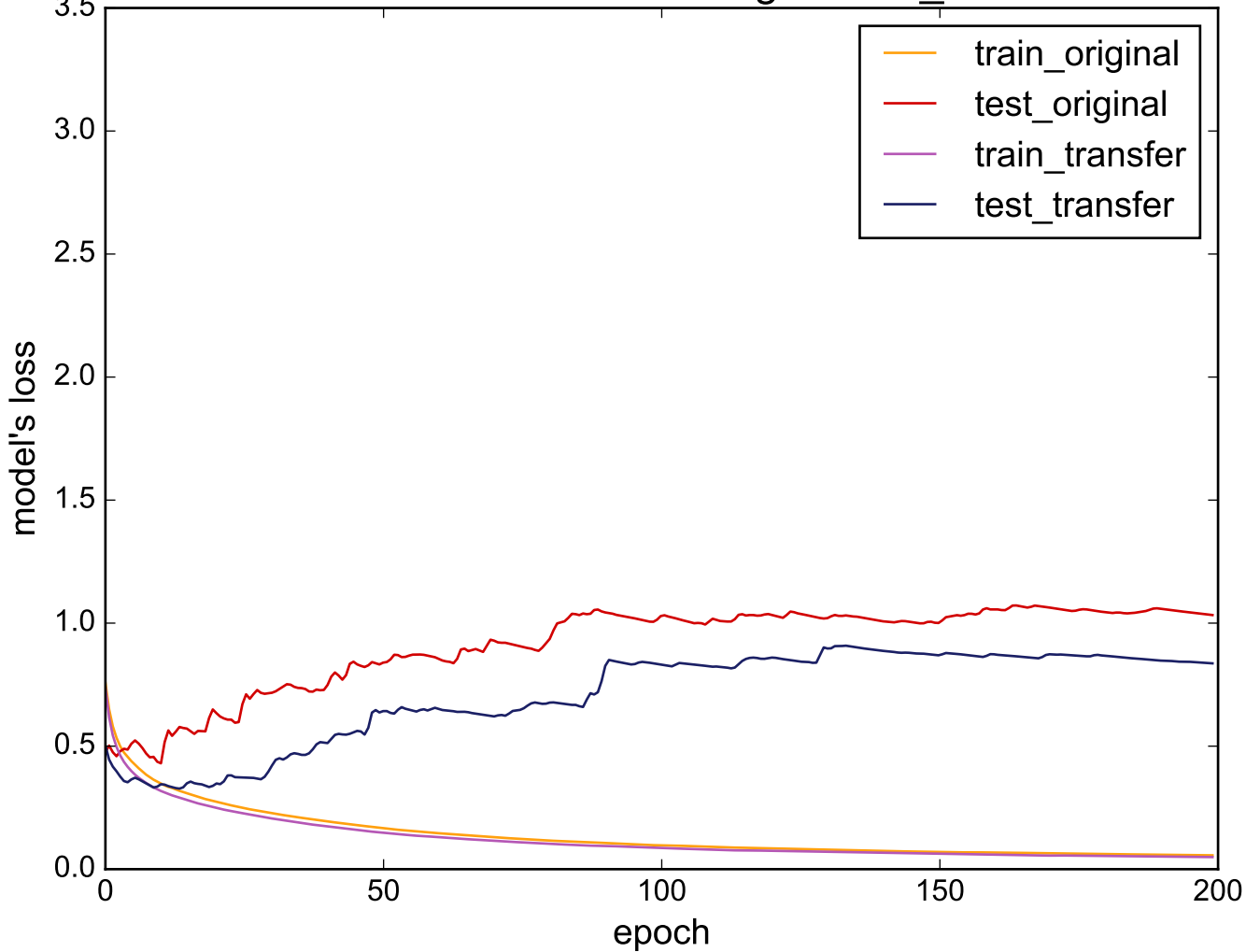
Source: TwoLeadECG - Target: Two_Patterns
