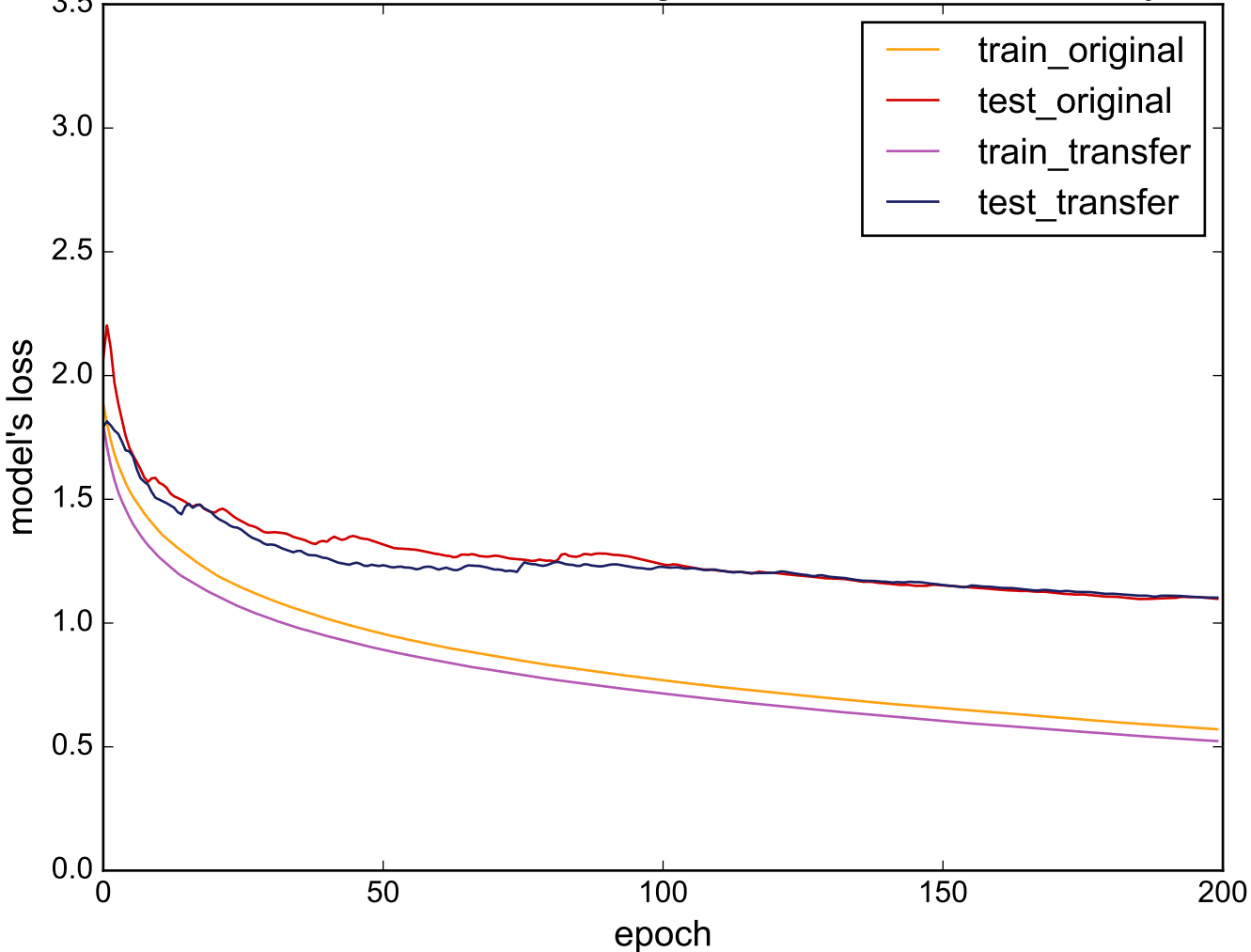
Source: TwoLeadECG - Target: UWaveGestureLibraryAll
