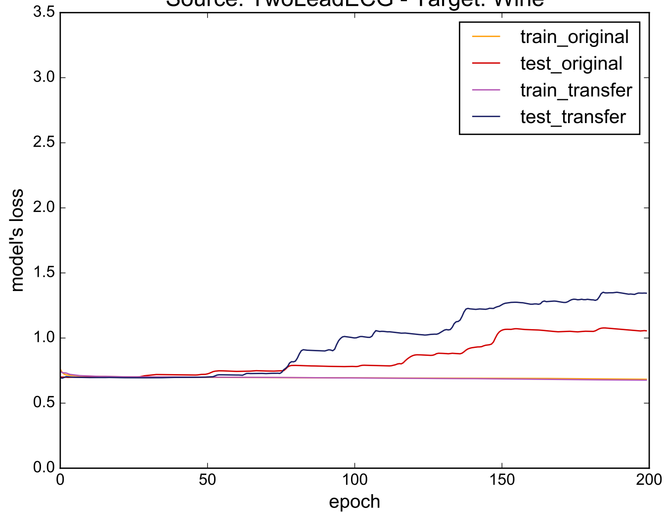
Source: TwoLeadECG - Target: Wine
