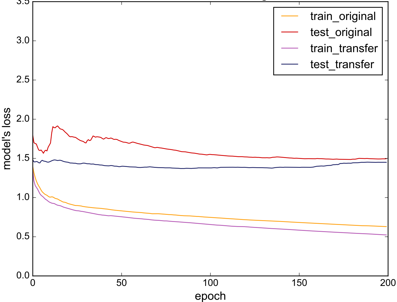
Source: TwoLeadECG - Target: Worms
