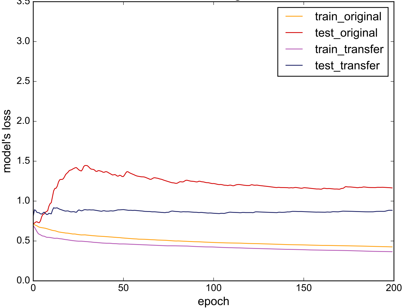
Source: TwoLeadECG - Target: WormsTwoClass
