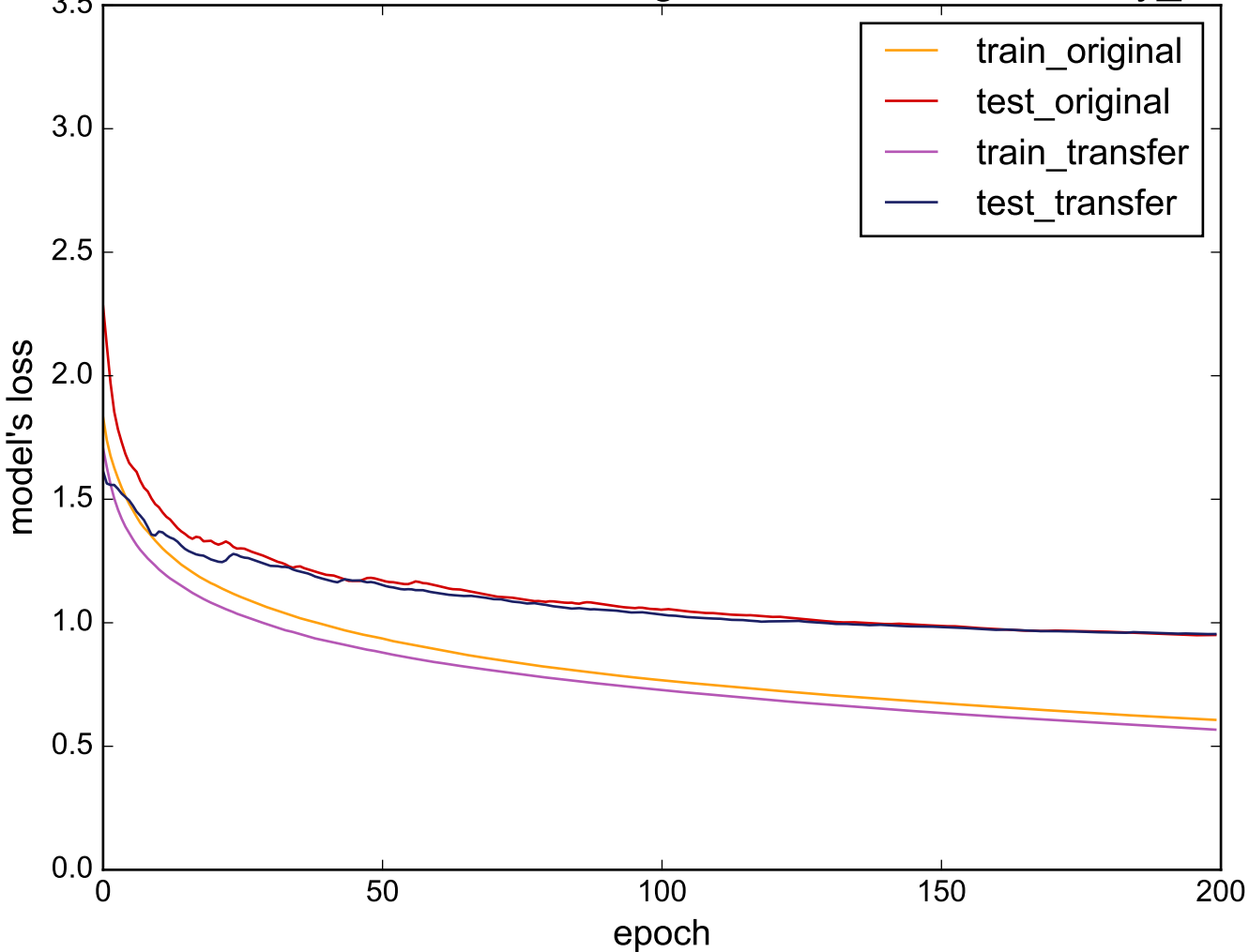
Source: TwoLeadECG - Target: uWaveGestureLibrary_X
