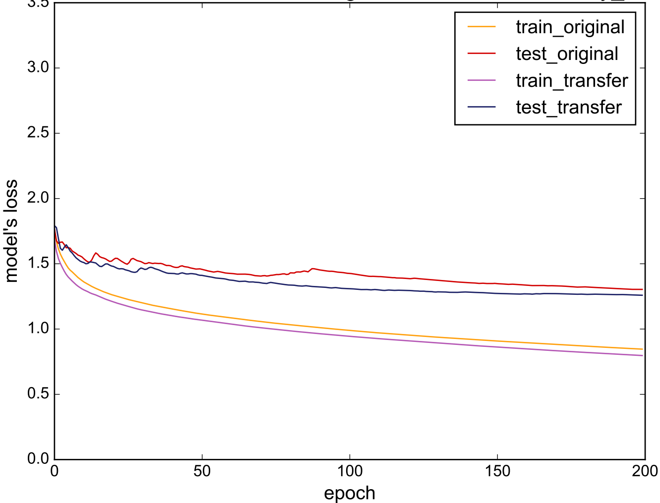
Source: TwoLeadECG - Target: uWaveGestureLibrary_Y
