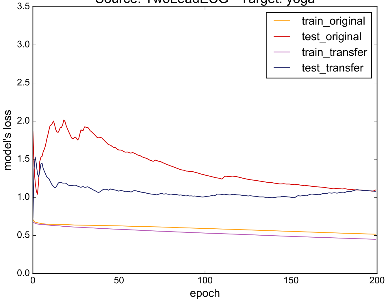
Source: TwoLeadECG - Target: yoga
