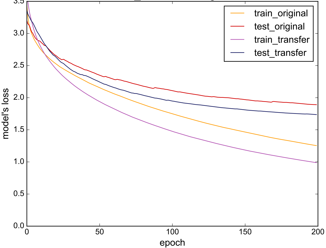
Source: Two_Patterns - Target: 50words
