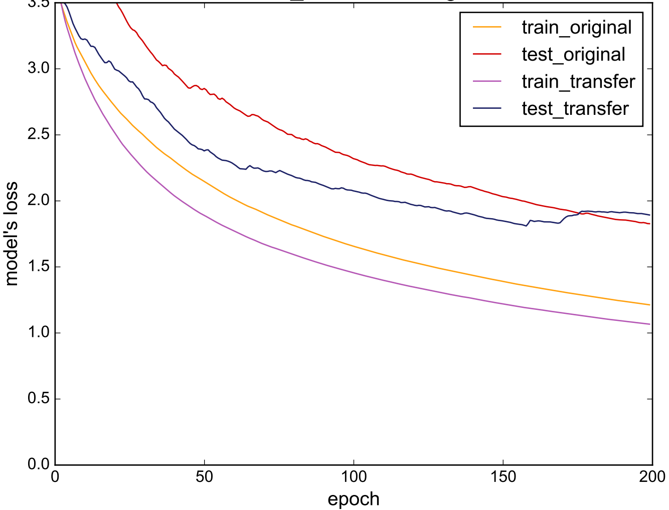
Source: Two_Patterns - Target: Adiac
