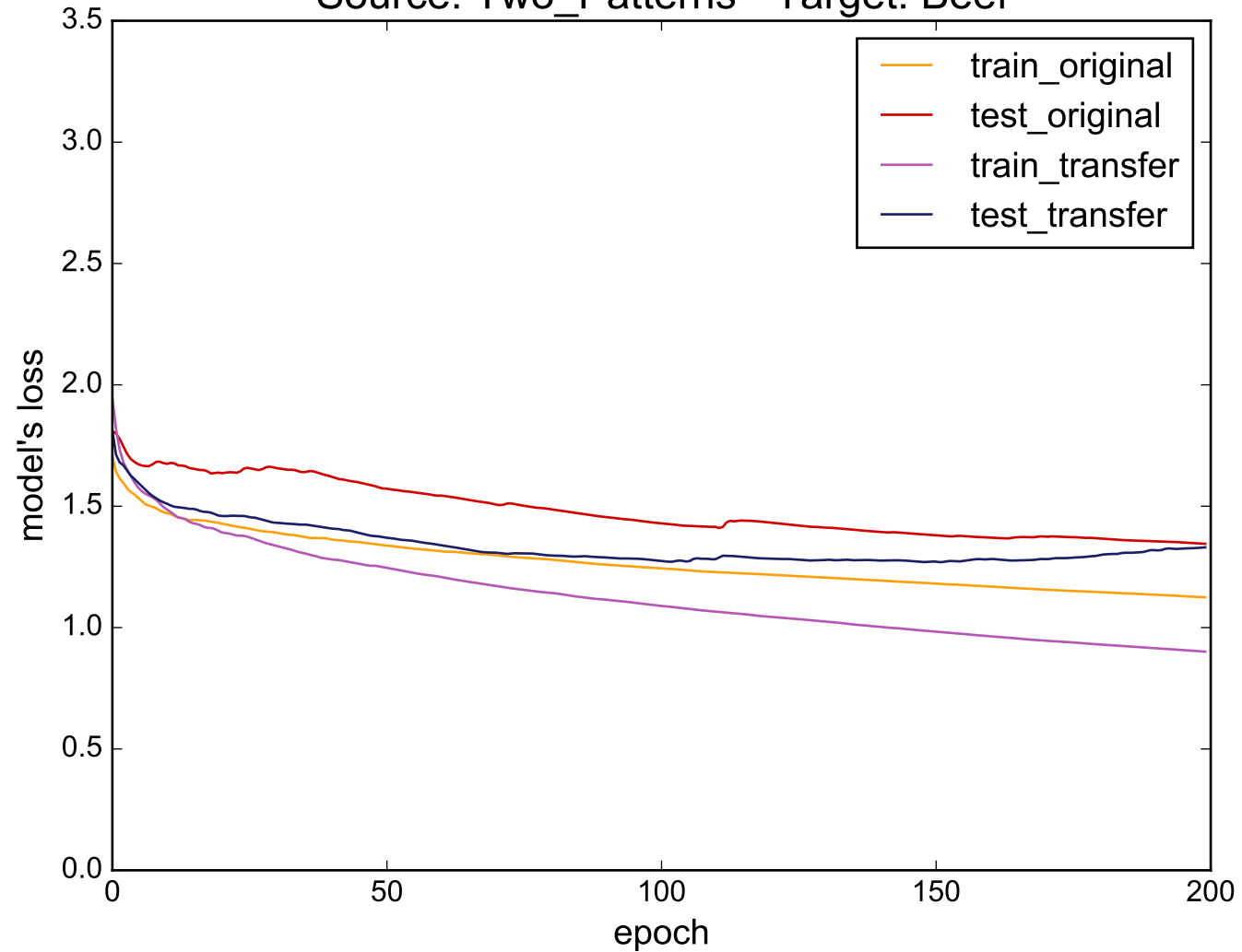
Source: Two_Patterns - Target: Beef
