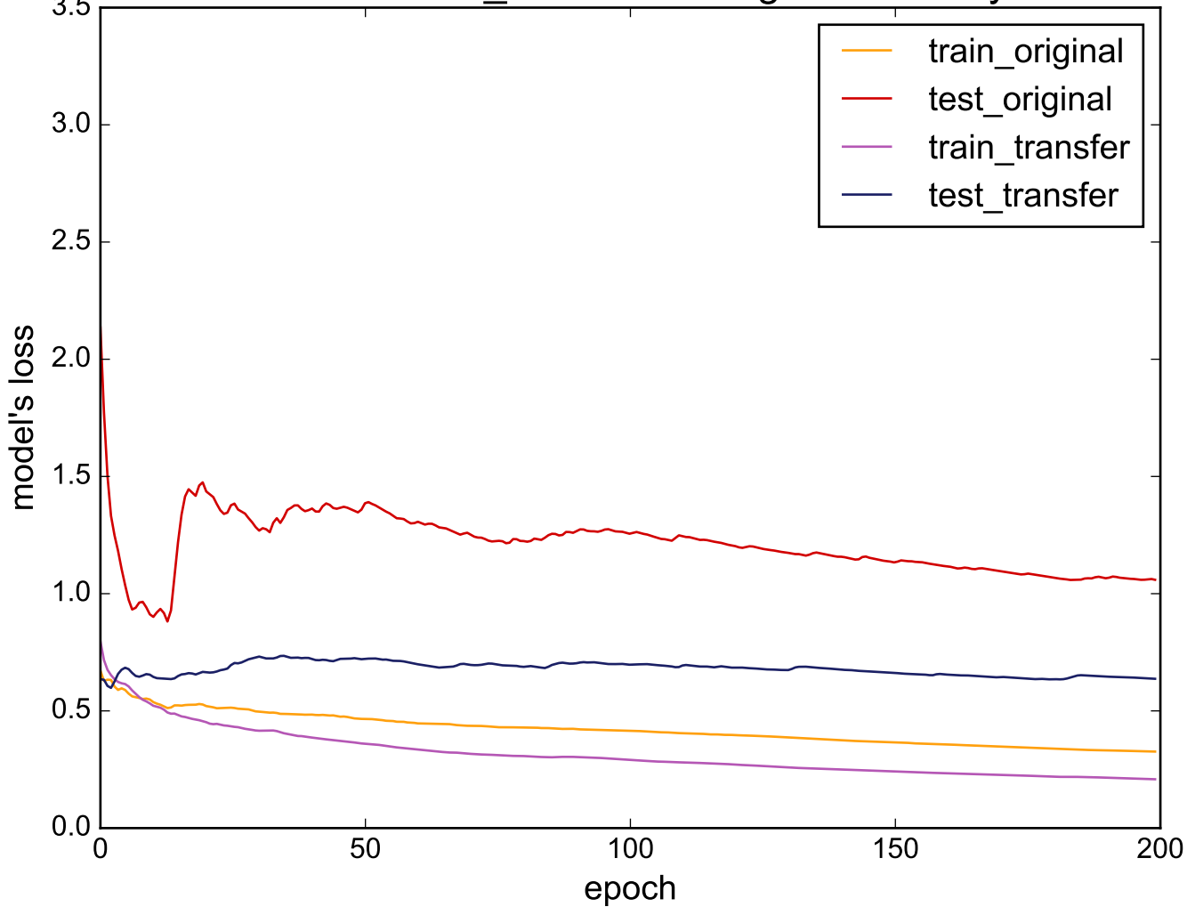
Source: Two_Patterns - Target: BeetleFly
