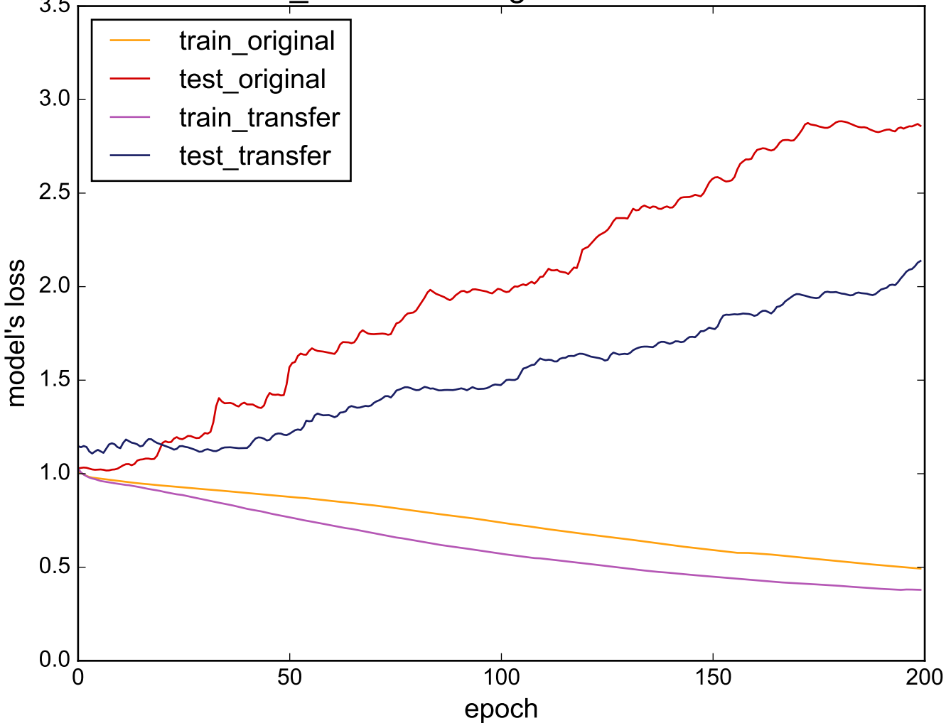
Source: Two_Patterns - Target: ChlorineConcentration
