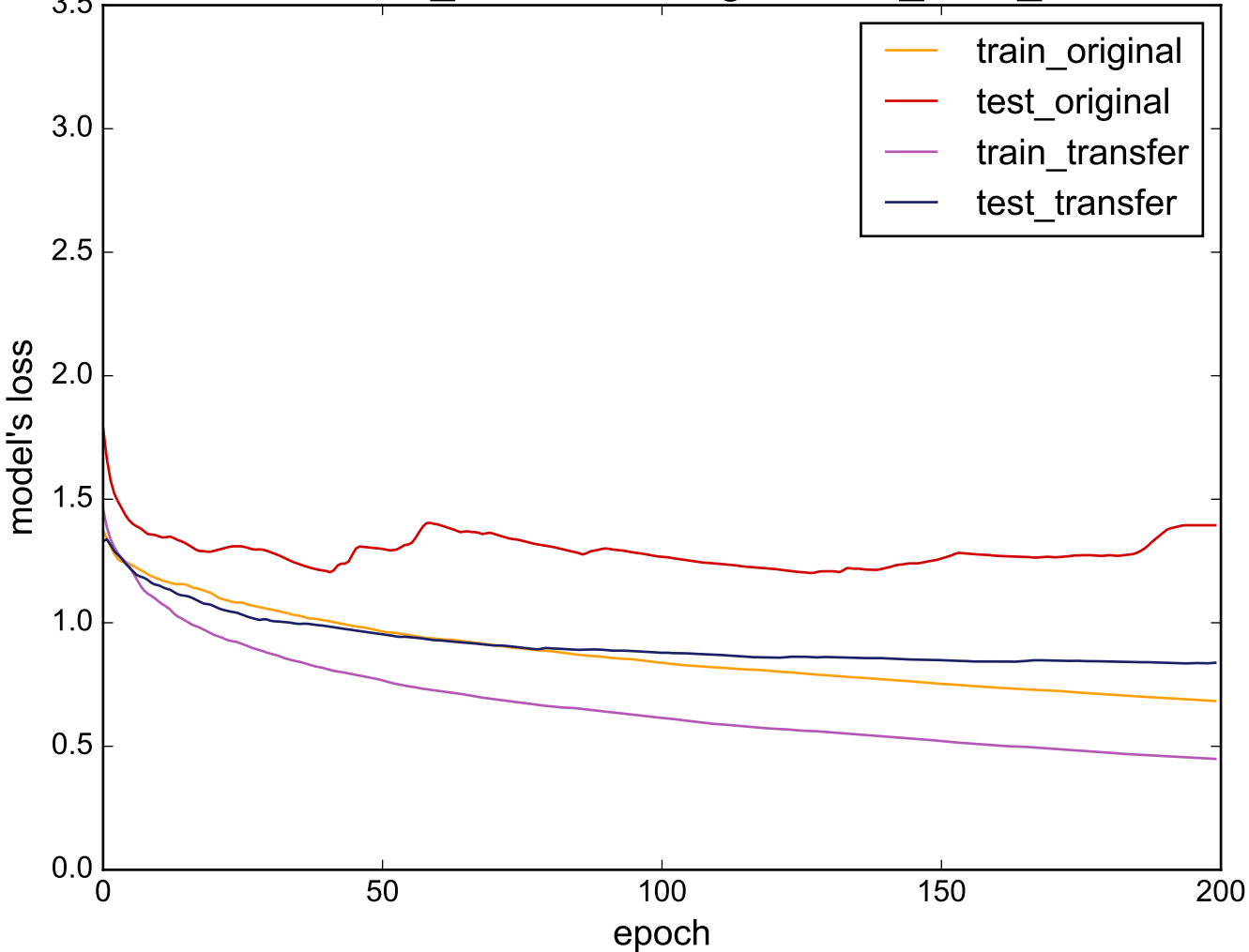
Source: Two_Patterns - Target: CinC_ECG_torso
