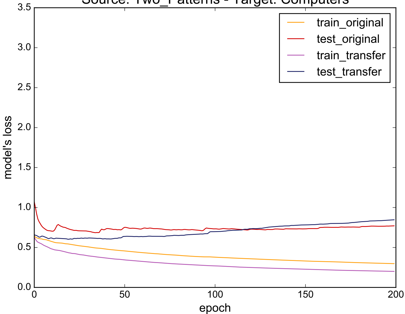
Source: Two_Patterns - Target: Computers
