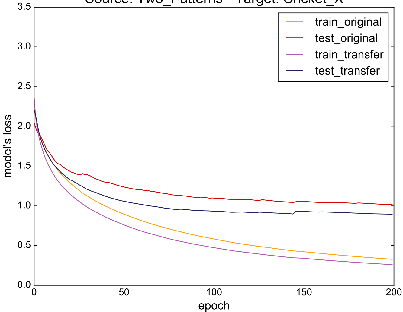
Source: Two_Patterns - Target: Cricket_X
