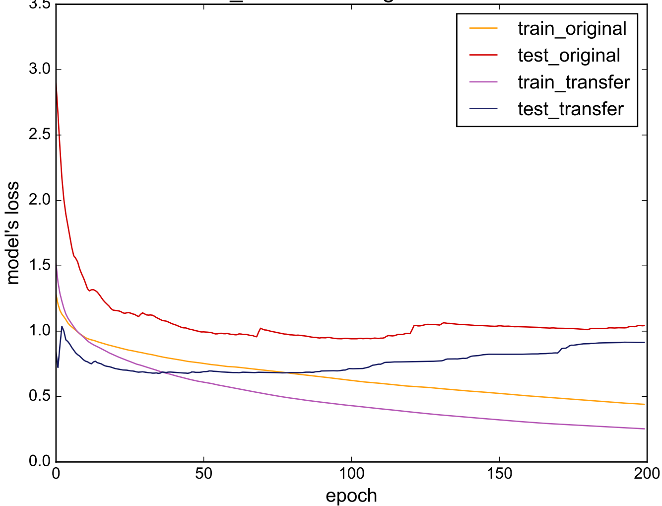
Source: Two_Patterns - Target: DistalPhalanxTW
