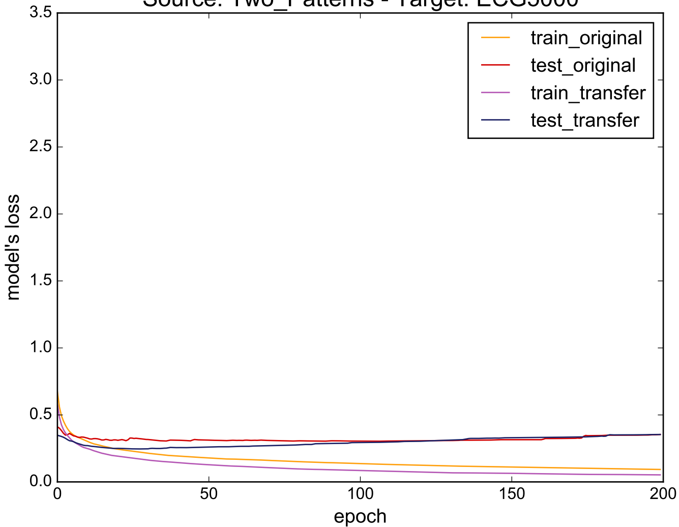
Source: Two_Patterns - Target: ECG5000
