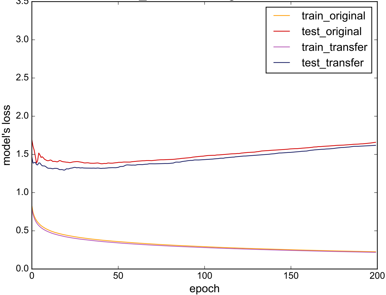
Source: Two_Patterns - Target: ElectricDevices
