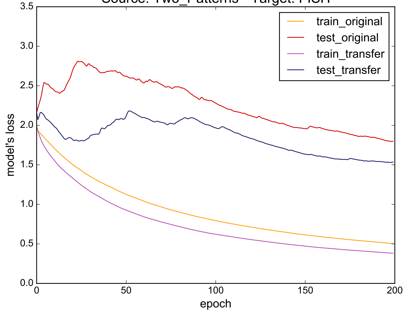
Source: Two_Patterns - Target: FISH
