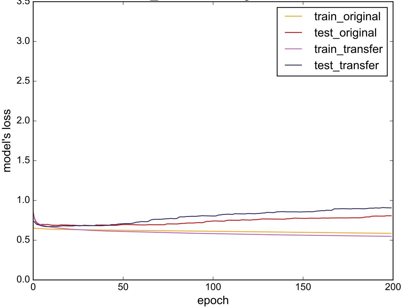
Source: Two_Patterns - Target: HandOutlines
