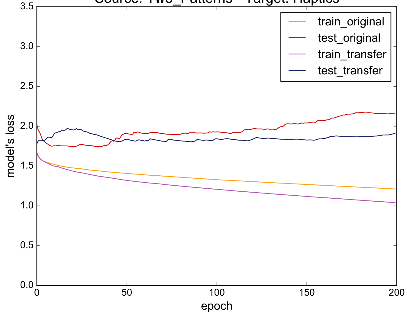
Source: Two_Patterns - Target: Haptics
