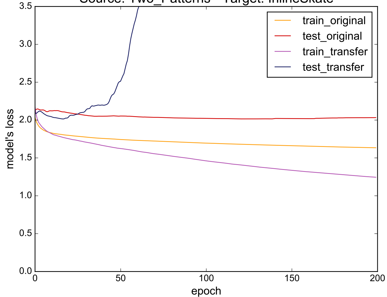
Source: Two_Patterns - Target: InlineSkate
