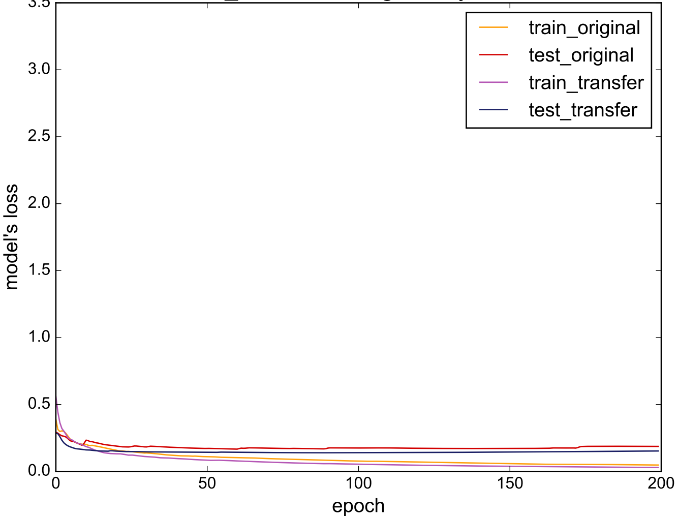
Source: Two_Patterns - Target: ItalyPowerDemand
