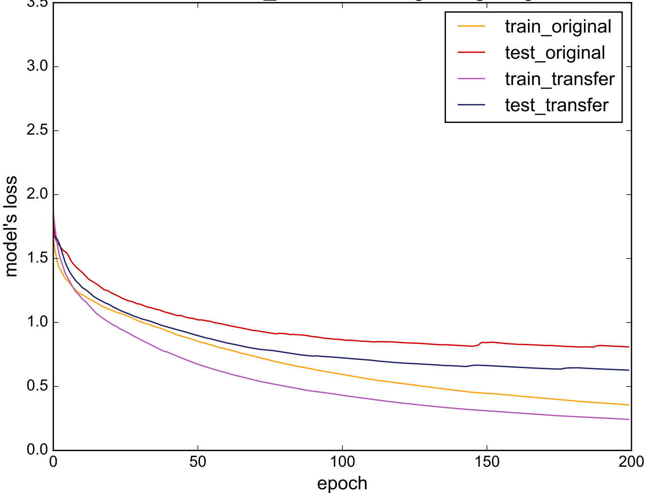
Source: Two_Patterns - Target: Lighting7
