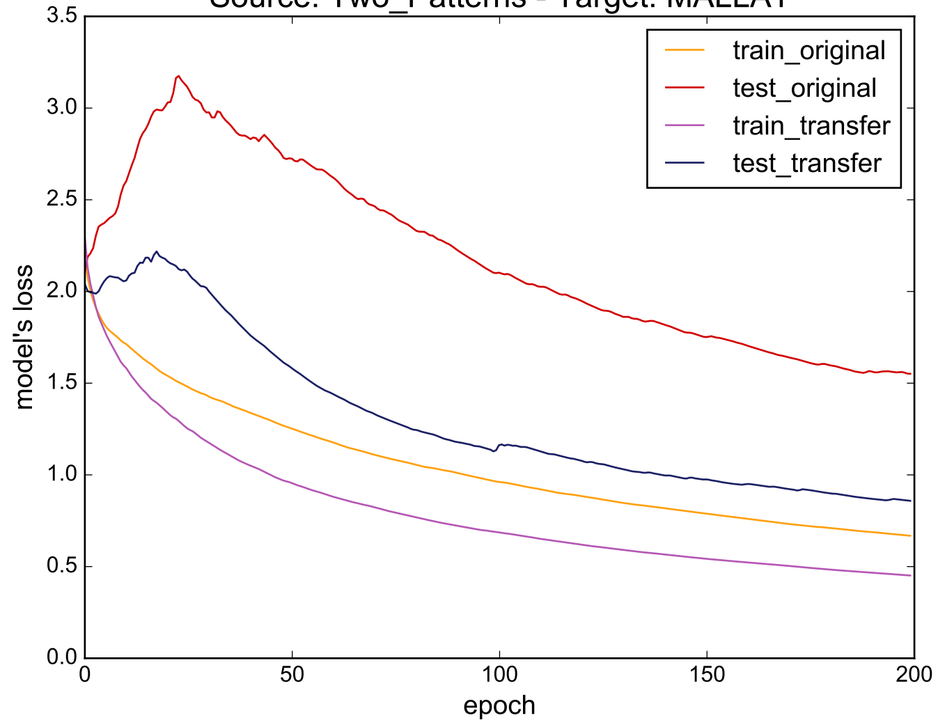
Source: Two_Patterns - Target: MALLAT
