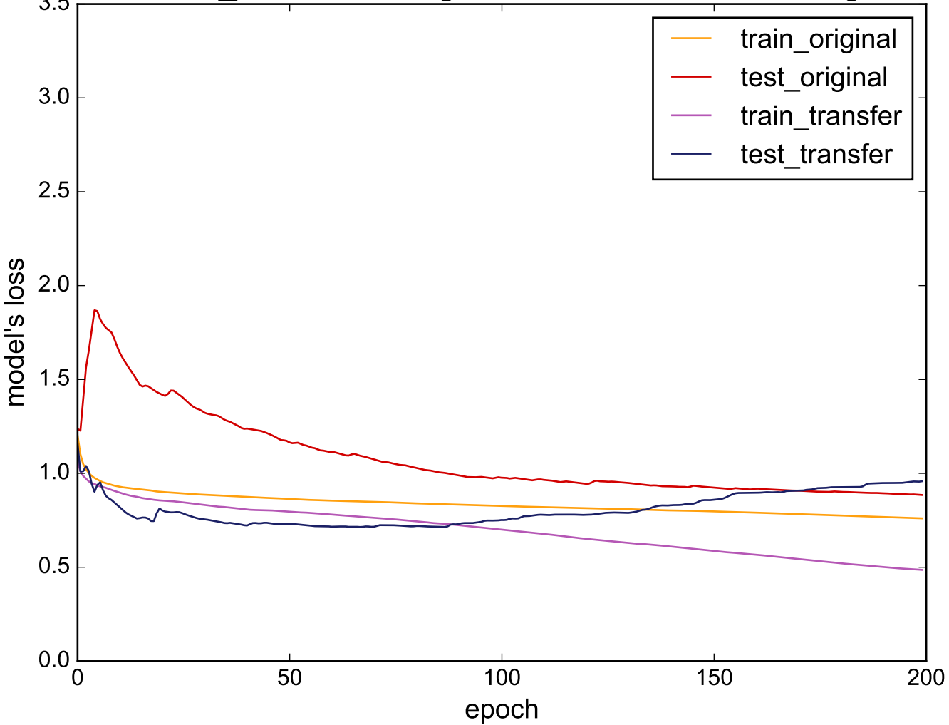
Source: Two_Patterns - Target: MiddlePhalanxOutlineAgeGroup
