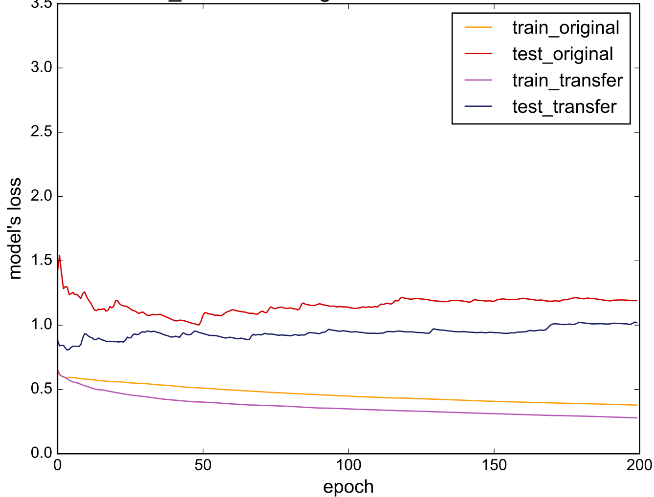
Source: Two_Patterns - Target: MiddlePhalanxOutlineCorrect
