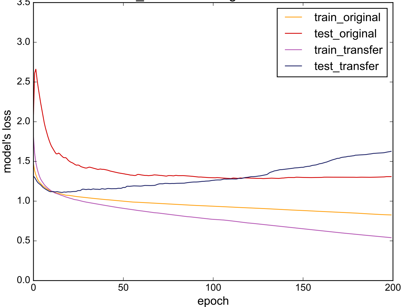
Source: Two_Patterns - Target: MiddlePhalanxTW
