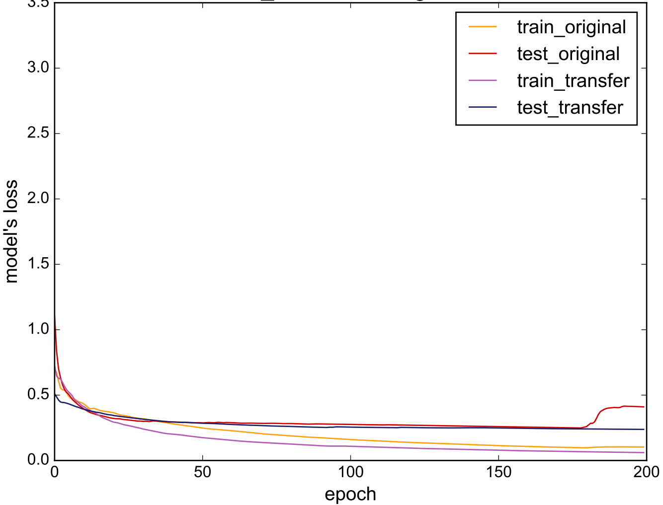
Source: Two_Patterns - Target: MoteStrain
