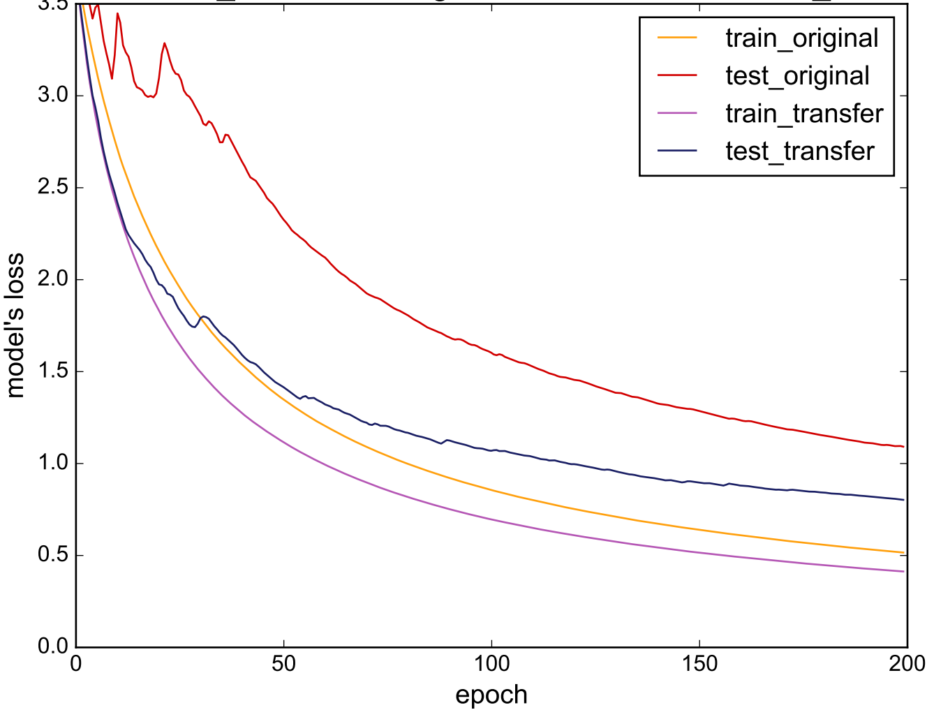
Source: Two_Patterns - Target: NonInvasiveFetalECG_Thorax1
