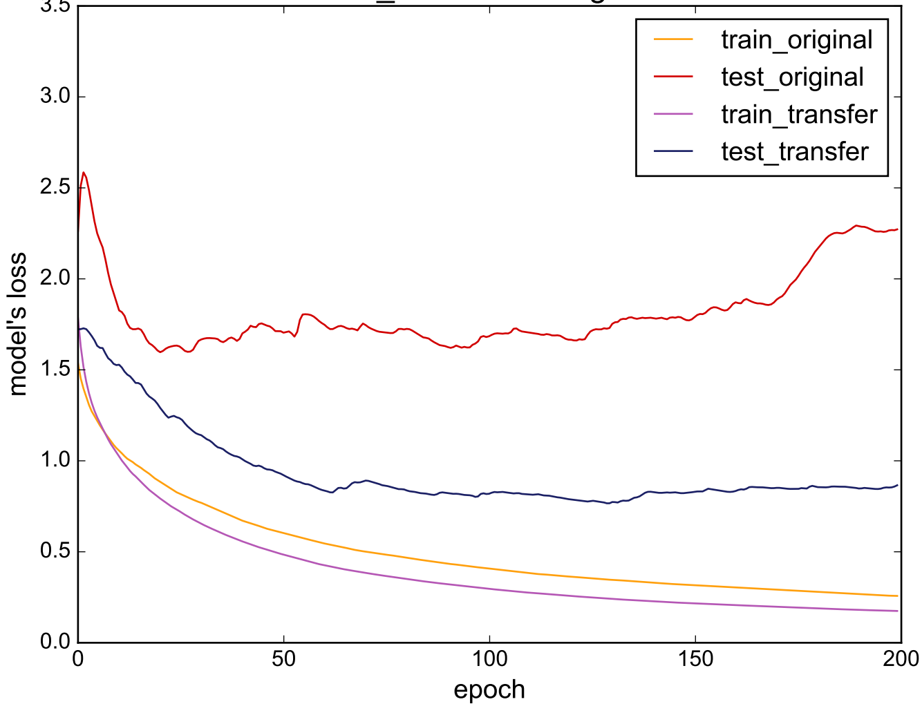
Source: Two_Patterns - Target: OSULeaf
