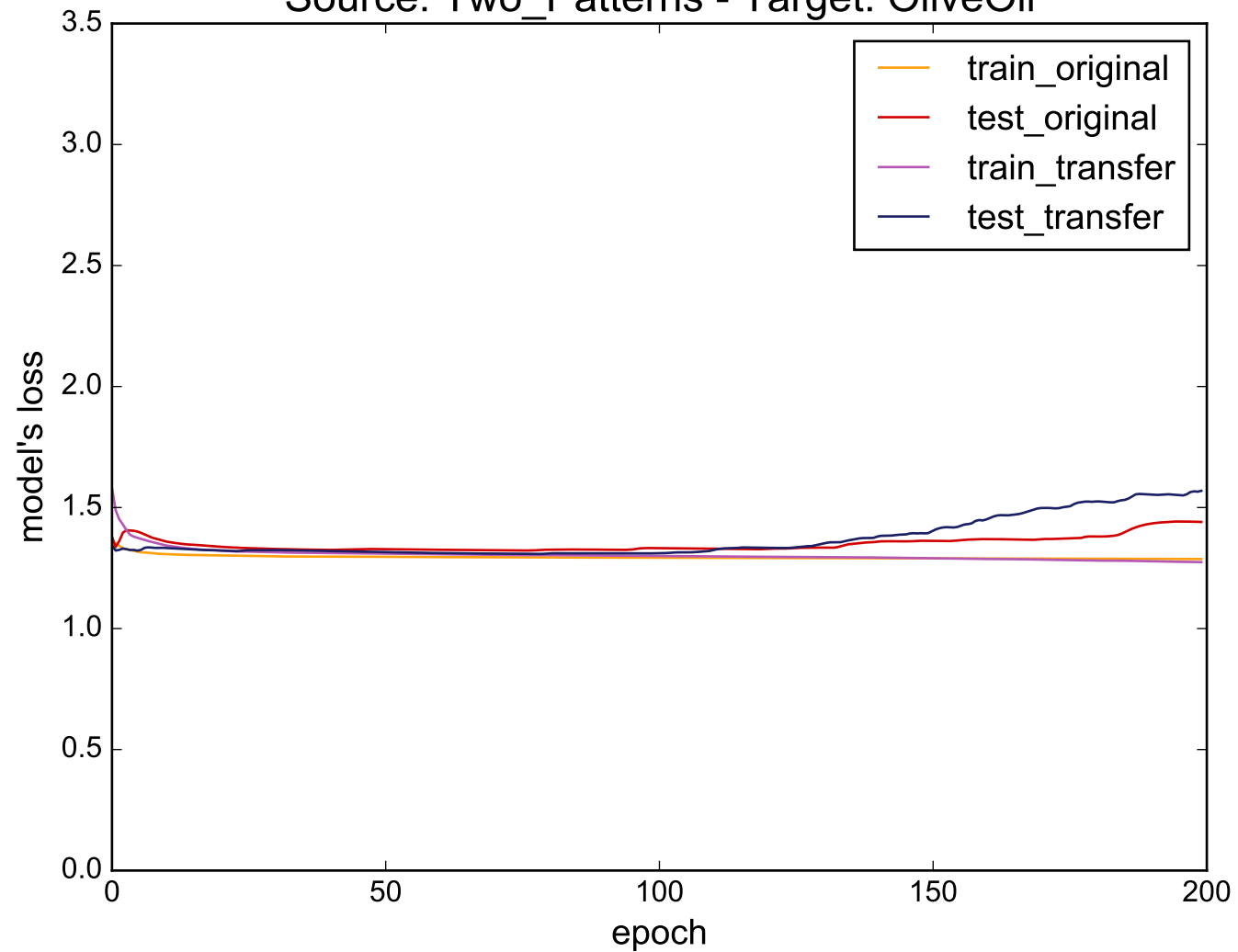
Source: Two_Patterns - Target: OliveOil
