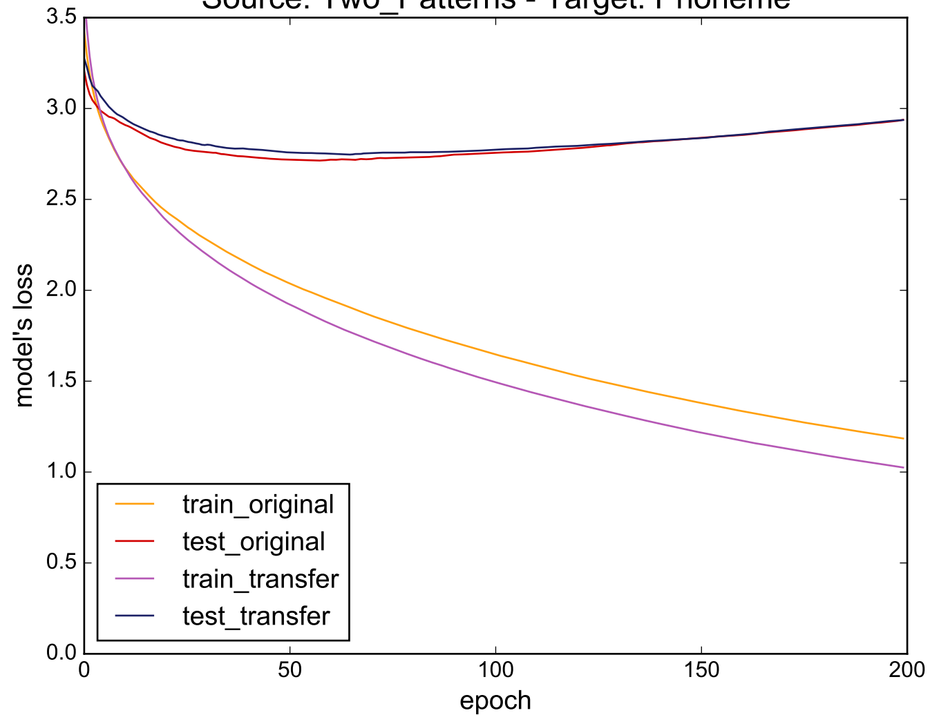
Source: Two_Patterns - Target: Phoneme
