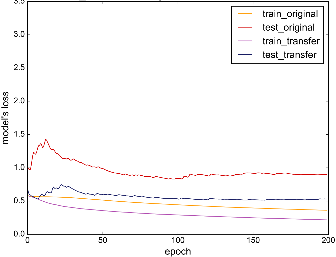
Source: Two_Patterns - Target: ProximalPhalanxOutlineCorrect
