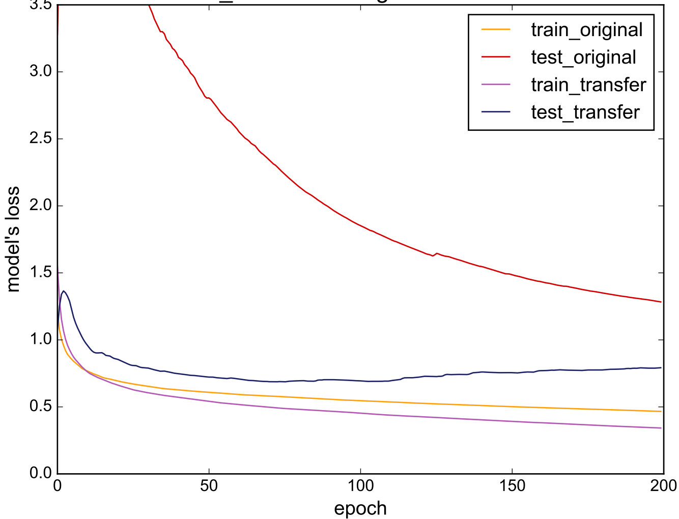
Source: Two_Patterns - Target: ProximalPhalanxTW
