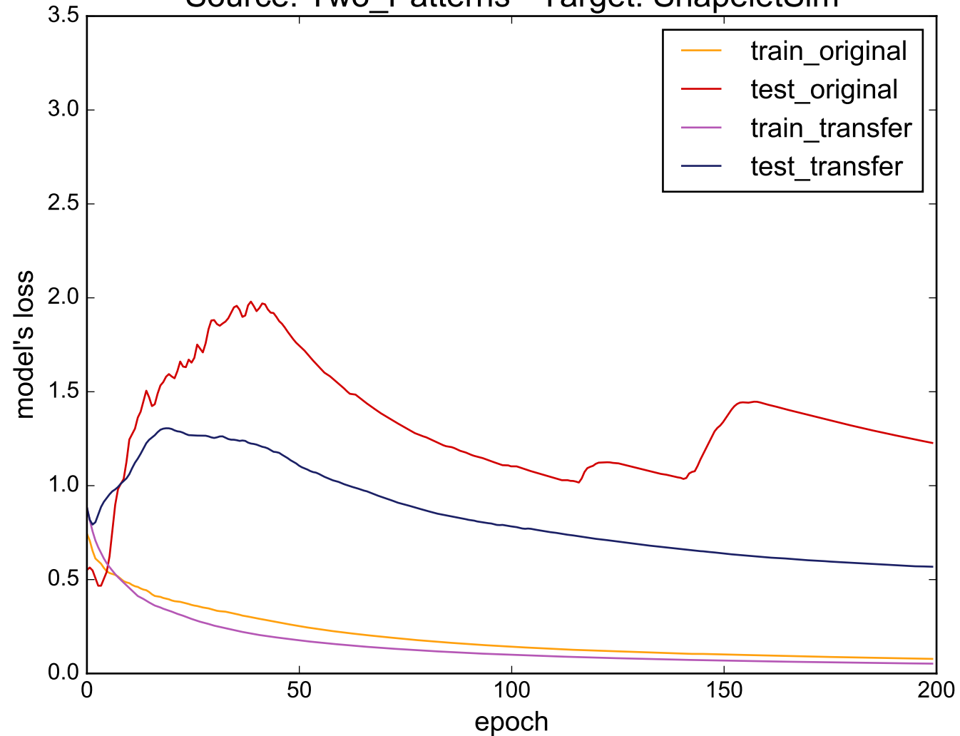
Source: Two_Patterns - Target: ShapeletSim
