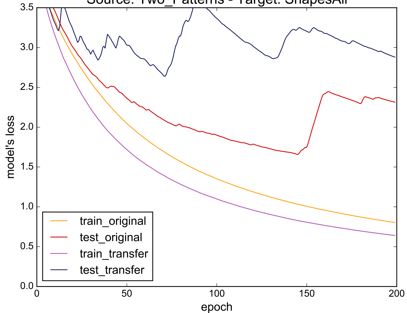
Source: Two_Patterns - Target: ShapesAll
