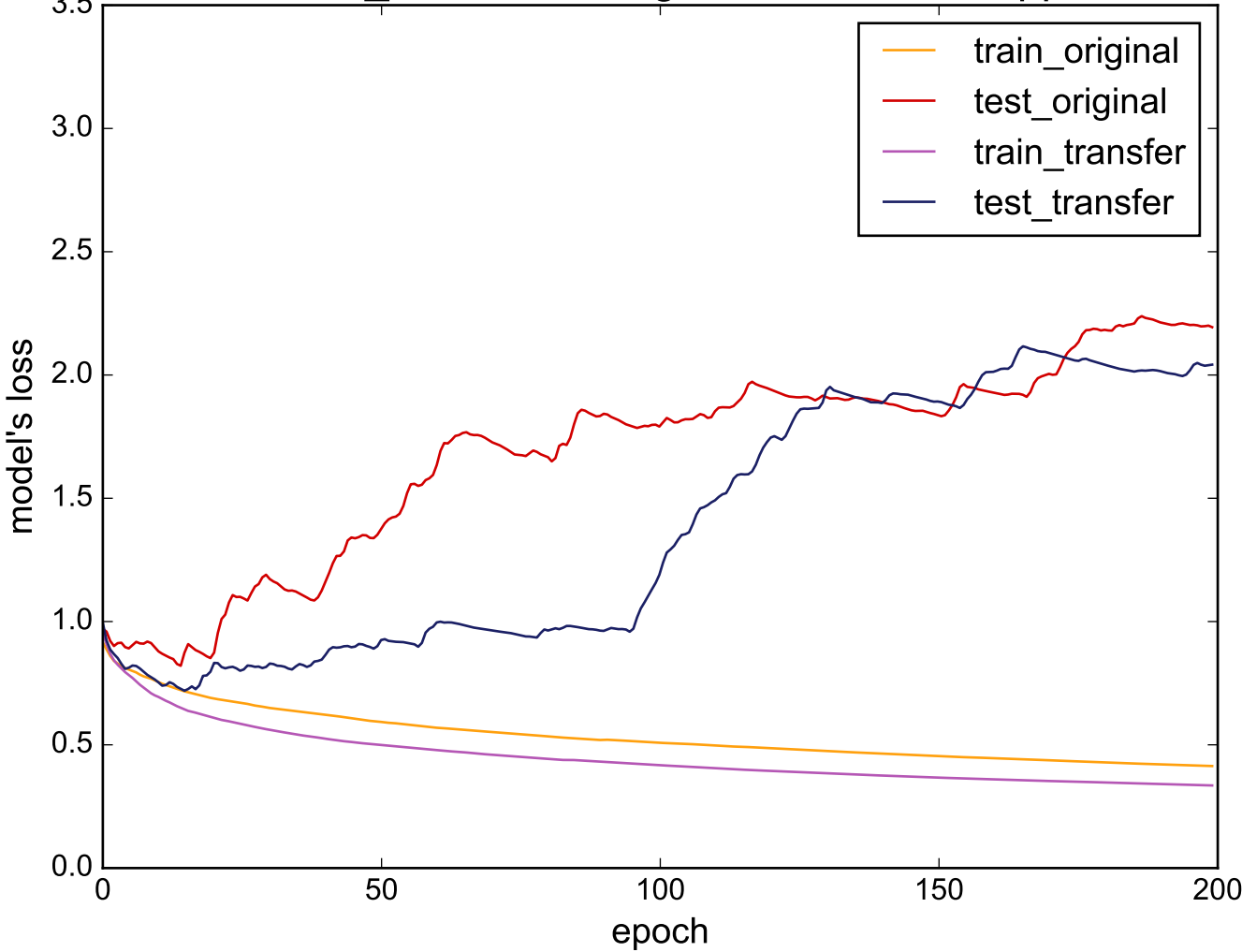
Source: Two_Patterns - Target: SmallKitchenAppliances
