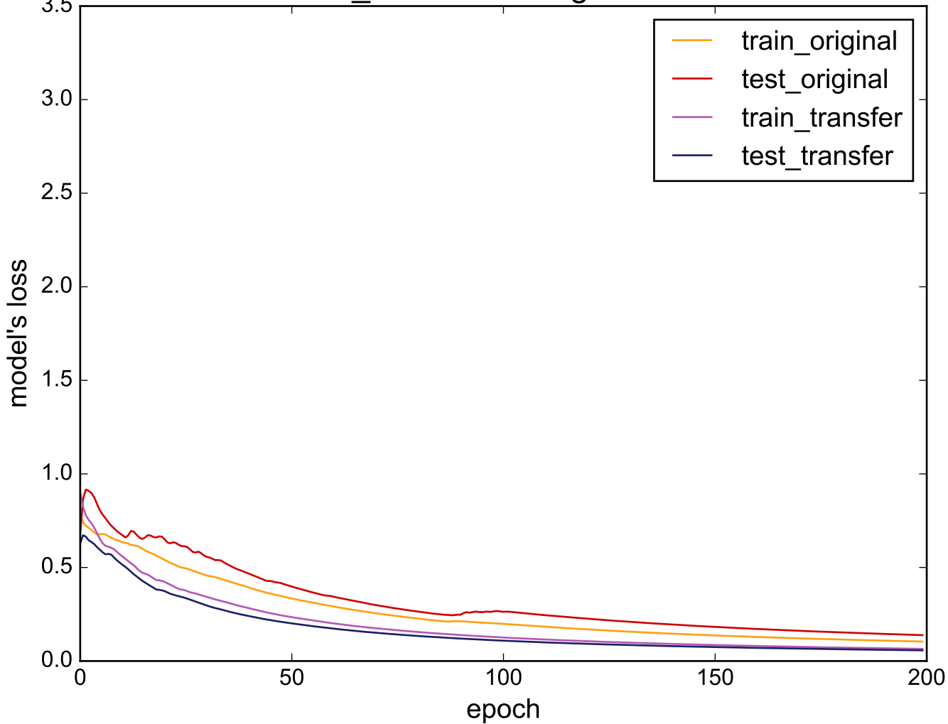
Source: Two_Patterns - Target: TwoLeadECG
