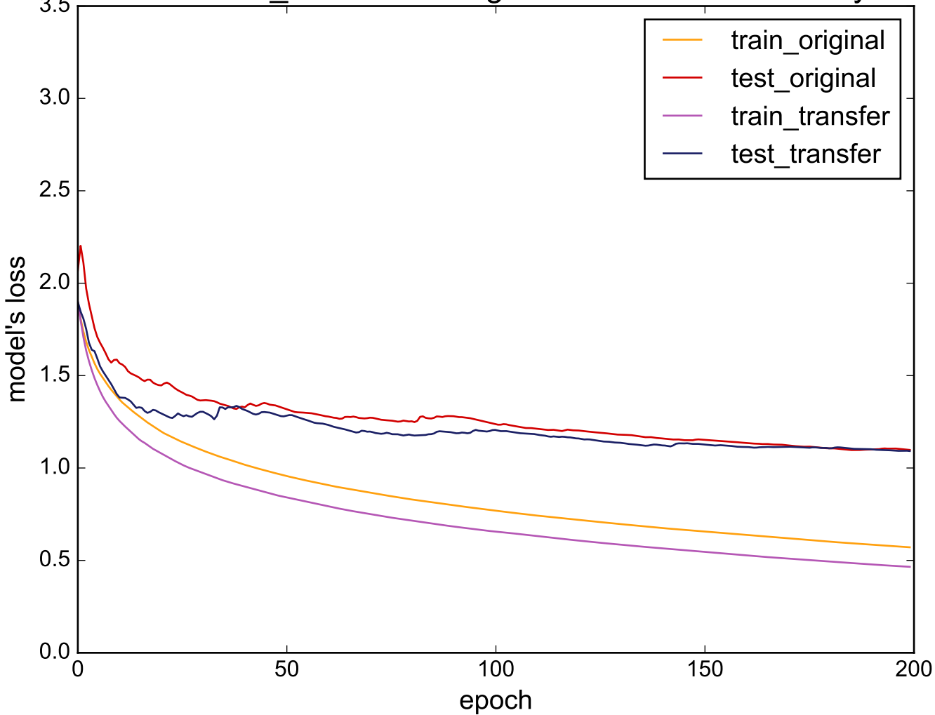
Source: Two_Patterns - Target: UWaveGestureLibraryAll
