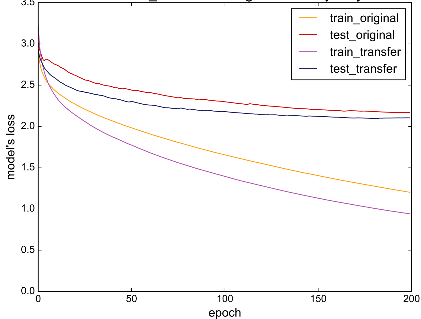
Source: Two_Patterns - Target: WordsSynonyms
