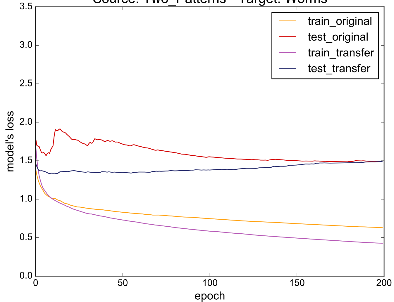
Source: Two_Patterns - Target: Worms
