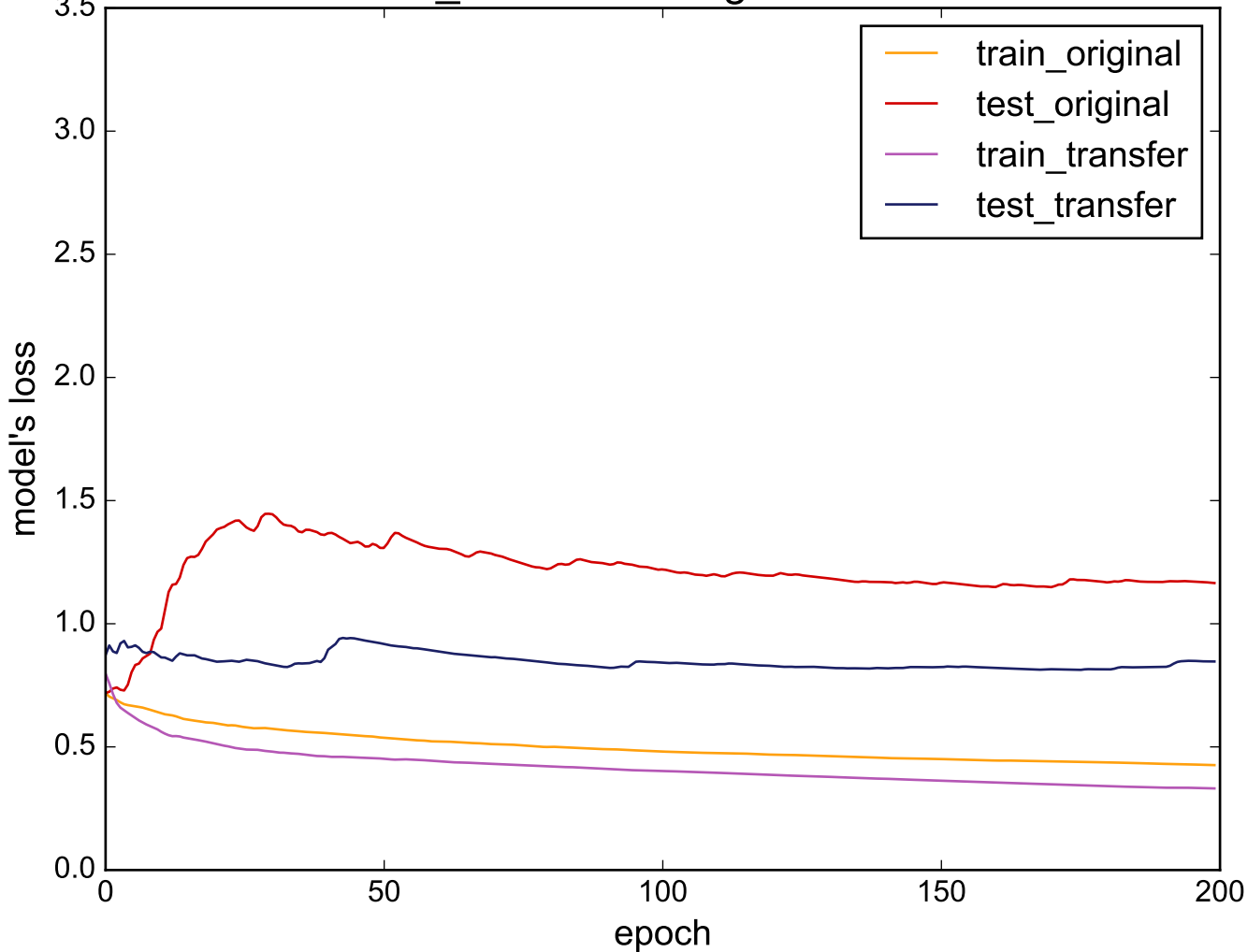
Source: Two_Patterns - Target: WormsTwoClass
